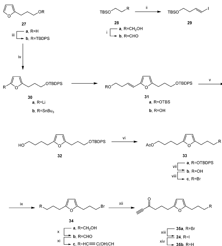
Scheme 4 Reagents and conditions: (i) PCC, silica, DCM, 4 h, 60%; (ii) \text{ICH}_2^+\text{PPh}_3\text{I}^- , \text{KO}^-\text{Bu} , THF, -60 \rightarrow -40 °C, 2 h, 97%; (iii) TBDPSCl, \text{NEt}_3 , DMAP, DCM, 16 h, 97%; (iv) (a) t\text{-BuLi} , THF, -78 \rightarrow -20 °C, 3 h, then \text{Bu}_3\text{SnCl} , -20 °C \rightarrow rt, 3 h, then 29 , \text{Pd}(\text{PPh}_3)_2\text{Cl}_2 , THF, 67 °C, 16 h, (b) PPTS, MeOH, 24 h, 40%; (v) \text{Pd}(\text{OH})_2 , \text{H}_2 , MeOH, 6 h, 96%; (vi) \text{Ac}_2\text{O} , \text{NEt}_3 , DMAP, DCM, 0 °C, 6 h, 74%; (vii) TBAF, THF, 2 h, 96%; (viii) \text{CBr}_4 , \text{PPh}_3 , DCM, 0 °C, 20 min, 95%; (ix) \text{K}_2\text{CO}_3 , MeOH, 4 h, 98%; (x) Dess–Martin periodinane, DCM, 20 min, 70%; (xi) \equiv\text{MgBr} , THF, 0 °C \rightarrow rt, 30 min, 84%; (xii) Dess–Martin periodinane, DCM, 30 min, 88%; (xiii) NaI, \text{K}_2\text{CO}_3 , acetone, 14 h, quant.; (xiv) \text{Et}_3\text{B} , \text{Bu}_3\text{SnH} , Tol, 0 °C, 48 h, 37%.
