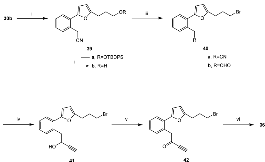
Scheme 5 Reagents and conditions: (i) 2-iodobenzeneacetonitrile, Pd(PPh 3 ) 2 Cl 2 , THF, 67 °C, 16 h, 89%; (ii) TBAF, p TSA, THF, 12 h, 75%; (iii) CBr 4 , PPh 3 , DCM, 0 °C, 30 min, 85%; (iv) (a) DIBAL-H, Tol, -78 → 0 °C, 4.5 h, (b) ≡-MgBr, THF, -78 °C → rt, 2h, 60%; (v) Dess–Martin periodinane, DCM, 2 h, 50%; (vi) NaI, K 2 CO 3 , acetone, 14 h, 77%.
